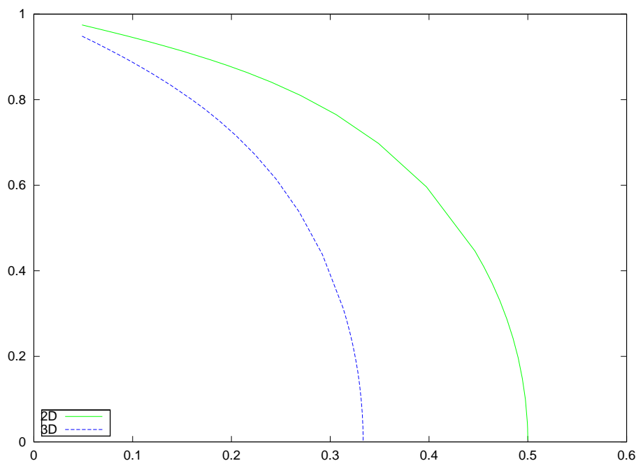
Figure 1: Graph of c(\kappa(\sigma)) against \sigma
