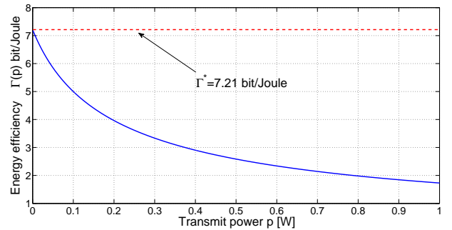
Fig. 2. Type II energy-efficiency vs. transmit power p .
