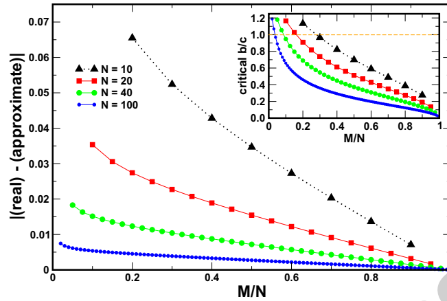
Figure 3: In the main panel we compare the numerical solution of \bar{x} with the asymptotic approximation in Eq. (9), for different values of M/N and group sizes N = 10, 20, 40 and 100 . In the inset we plot the critical value of b/c as a function of M/N for the same group sizes; for small M/N , the critical value behaves conventionally in the sense that b > c , cooperation being feasible only when the benefit outweighs the cost. With increasing M/N , however, we observe a decrease of the critical benefit-to-cost ratio b/c (see main text for details).
