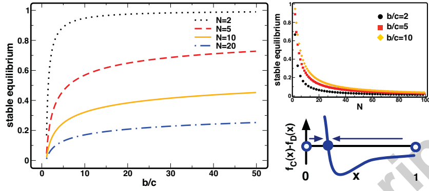
Figure 1: Stable equilibria of the N -person SG in infinite populations. In the main panel we show the location of the stable interior equilibrium of the replicator dynamics equation as a function of the benefit-to-cost ratio b/c for group sizes N=2 (dotted black line), 5 (dashed red line), 10 (solid yellow line) and 20 (dash-dot blue line). The stable nature of this interior fixed point is illustrated in the inset on the lower right. In the small panel in the upper right we show how the location of the interior stable fixed point scales with group size for the three different benefit-to-cost ratios b/c indicated.
