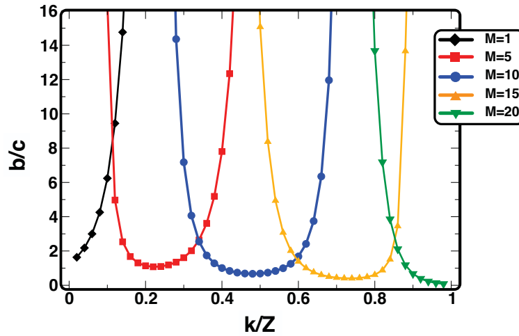
Figure 4: Equilibria of the N -person snowdrift game with threshold in finite populations. Population size is Z = 50 and group size is N = 20 . We vary the threshold M above which cooperation leads to a common benefit b . For each k/Z we show the corresponding b/c at which g(k) = 0 (cf. Eq. (13)). Whenever the population size is large compared to group size, selection in finite populations is qualitatively similar to that in infinite populations.
