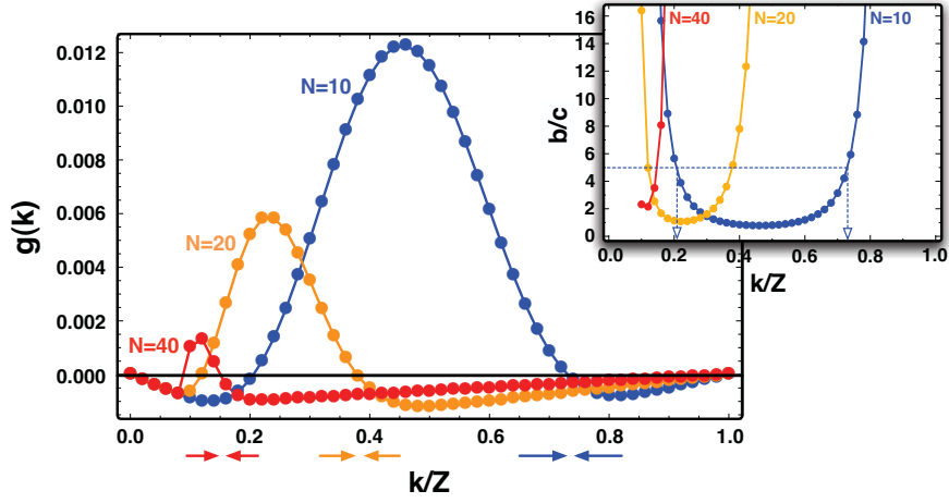
Figure 5: Effect of group size in the evolution of cooperation. In the main panel, we plot g(k) (defined in Eq. (13)) as a function of the fraction of cooperators k/Z , for b/c = 5 . We fixed the population size at Z = 50 and the threshold at M = 5 , while varying the group size N . As the group size approaches the population size, the range of values of k/Z for which cooperation is advantageous ( g(k) > 0 ) is reduced. In the inset, we show how the roots of g(k) vary with b/c for different values of the group size N . For N \sim Z the roots of g(k) disappear and defectors are always advantageous.
