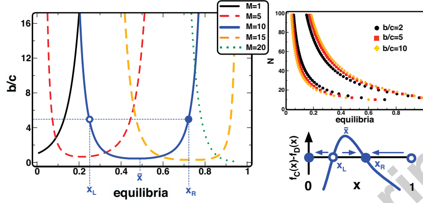
Figure 2: Equilibria of the N -person Snowdrift Game with threshold. We assume infinite, well-mixed populations, fix the group size at N = 20 and vary the threshold M above which cooperation leads to a common benefit b . The total cost involved is c . In the main panel we show how the occurrence of a threshold leads to the appearance of at most 2 interior fixed points x_L and x_R , which can be found via the intersection of a horizontal line with the appropriate curve (illustrated for M = 10 ); in this case, the leftmost root is always an unstable fixed point whereas the rightmost corresponds to stable fixed point, as illustrated in the small panel in the lower right (see main text for details). For a given M/N , there is a critical value \bar{\gamma} for the critical cost-to-benefit ratio c/b below which the 2 interior roots discussed above always exist. In the small panel (upper right) we show how these interior fixed points scale with variable group size N for some values of the b/c ratio indicated. For \bar{\gamma}b < c no interior fixed points exist and defectors dominate unconditionally, whereas for \bar{\gamma}b = c the only root corresponds to an unstable fixed point; it is noteworthy that \bar{\gamma} increases with increasing M/N (main panel) and can actually become larger than 1 (see main text for details).
