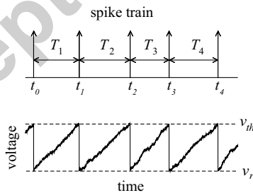
Figure 2: Subthreshold voltage dynamics and corresponding spike train as from a simulation of Eq. (7) and Eq. (8) (PIF) with parameters \mu = 0.9 and D = 0.006 . Note the high degree of regularity of the spike train, characteristic of the PIF model under strong mean input with low noise intensity.
