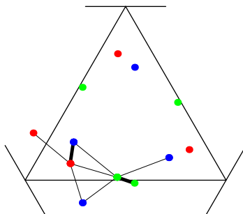
Figure 8: The protein positions and inter-protein bonds for MS2.
