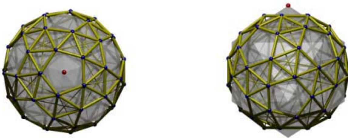
Figure 18: “Top” and “front” view of a geometric model of the capsid of STMV, including the inter-protein bonds. Dots denote the centre-of-mass positions of the protein chains, tubes denote bonds between them. This structure has 30 zero-modes without the A1-A8 bond (thin tubes); 24 of these are lifted by this weak bond.
