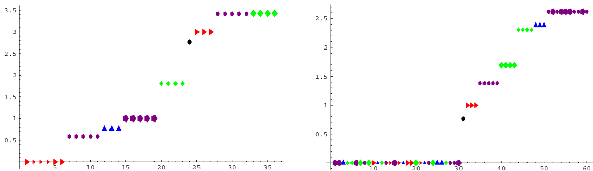
Figure 11: The spectrum of the icosahedron (left) and dodecahedron (right), decomposed in irreducible representations of the icosahedral group. Large symbols denote “-” representations, small symbols denote “+” representations. Black dots denote singlets, red triangles \Gamma_{3\pm} , blue triangles \Gamma_{3'\pm} , green squares \Gamma_{4\pm} and purple pentagons \Gamma_{5\pm} . Note that the structure of the non-zero modes is the same for both spring-mass models.
