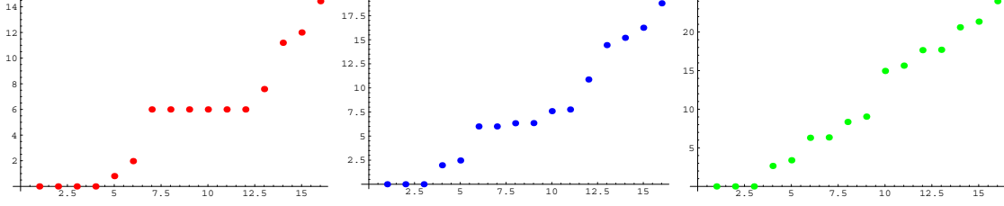
Figure 25: The exact frequency spectra for the Tirion potential with three different cutoffs, for the two protein chains' system.
