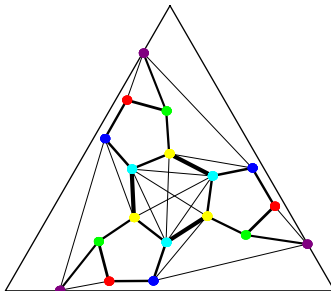
SV40 bonds on face
