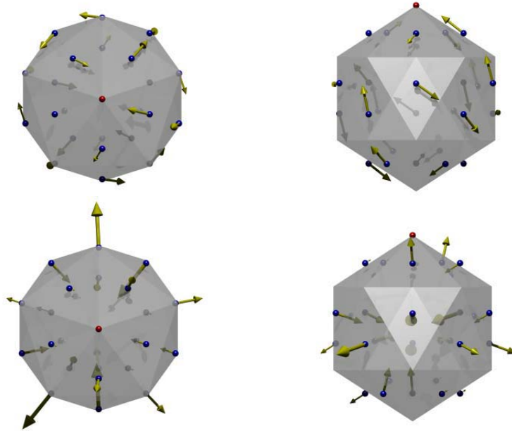
Figure 12: The zero-modes of the dodecahedron in the \Gamma_{3^+} (top) and \Gamma_{3^-} (bottom) representations.
