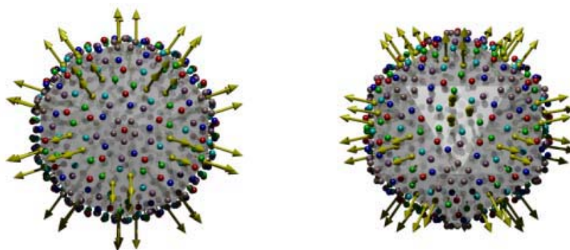
Figure 9: The first singlet mode of HK97, viewed along a 5-fold symmetry axis (left) and along a 3-fold axis (right). It occurs at position 67 with our particular bond choices, which is arguably still within the regime of the low-frequency approximation. This mode exhibits protrusion of the hexamer units (or rather, one of the chains of the hexamer), as also found in [46].
