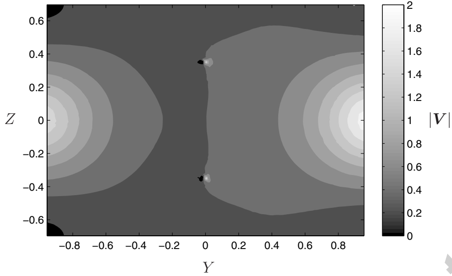
Fig. 7. The magnitude of the dimensionless Darcy velocity in the plane X = 0.3 in configuration A with \mathcal{Q} = 0.2 . Other details as in Fig. 6. Flow is generally from left to right, and fluid is emitted by the fibres.
