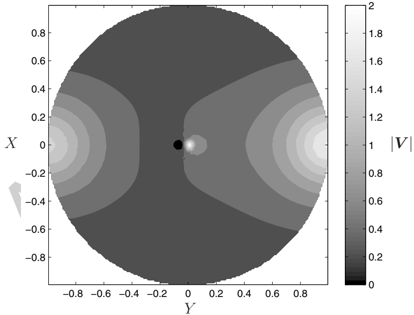
Fig. 10. The magnitude of the Darcy velocity in the plane Z = 0.3 in configuration B with \mathcal{Q} = 0.2 . Other details as in Fig. 9. Flow is generally from left to right, with fluid emitted by the fibre.
