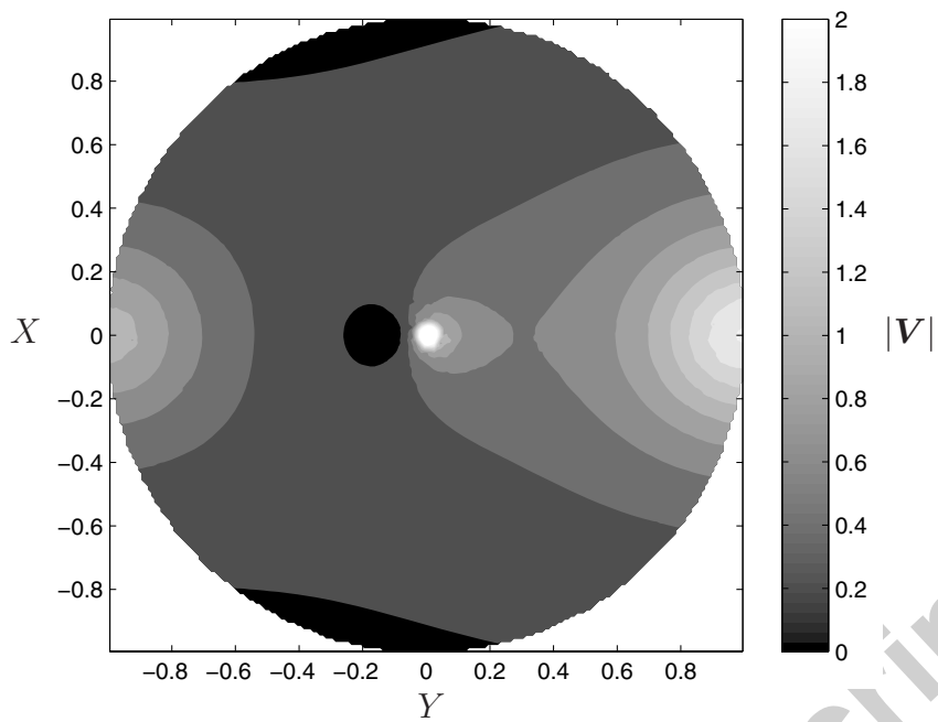
Fig. 11. The magnitude of the Darcy velocity in the plane Z = 0.3 in configuration B with \mathcal{Q} = 0.4 . Other details as in Fig. 9. Flow is generally from left to right, with fluid emitted by the fibre.
