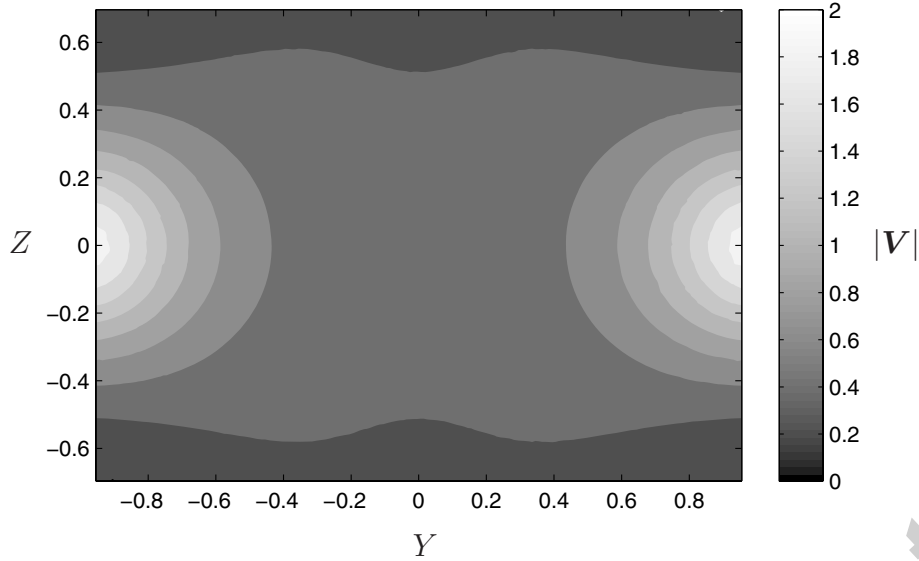
Fig. 6. The magnitude of the dimensionless Darcy velocity \mathbf{V} in the vertical plane X = 0.3 in configuration A with \mathcal{Q} = 0 (i.e. no flux from the fibres). The inlet is out of the plane to the left, and the outlet lies similarly to the right. The two fibres run perpendicular to the plane through Y = 0 , Z = \pm 0.35 . From the dimensionless Darcy velocity, the dimensional equivalent can be recovered from (10), and an estimate for the shear stress found using (58).
