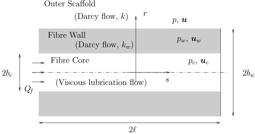
Fig. 5. The geometry of the porous-walled fibres, together with the coordinates and variables used to describe the flow within them.
