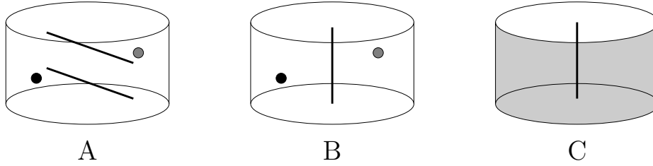
Fig. 4. Sketches of the bioreactor chamber, showing the three configurations of inlet/outlet pipes (filled circles) and porous fibres (thick lines) considered here. A more detailed view of configuration A is shown in Fig. 3. In configuration C, the whole of the cylindrical surface acts as a distributed outlet.
