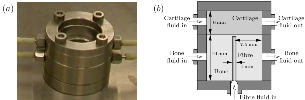
Fig. 1. A photograph (a) and sketch (b) of the two-chamber modular bioreactor, set up for configuration B (see §2). The tubes to the left and right provide flow to and from the inlet and outlet pipes, and porous fibre can be inserted through the base.
