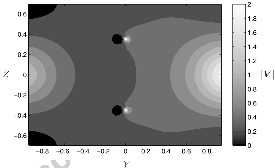
Fig. 8. The magnitude of the dimensionless Darcy velocity in the plane X = 0.3 in configuration A with \mathcal{Q} = 0.4 . Other details as in Fig. 6. Flow is generally from left to right, and fluid is emitted by the fibres.
