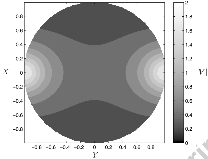
Fig. 9. The magnitude of the dimensionless Darcy velocity \mathbf{V} in the plane Z = 0.3 in configuration B with \mathcal{Q} = 0 (no flow from the fibre). The single fibre runs perpendicular to the plane, through X = Y = 0 . The inlet pipe is to the left and the outlet pipe to the right, both in the plane Z = 0 . From the dimensionless Darcy velocity, the dimensional equivalent can be recovered from (10), and an estimate for the shear stress found using (58).
