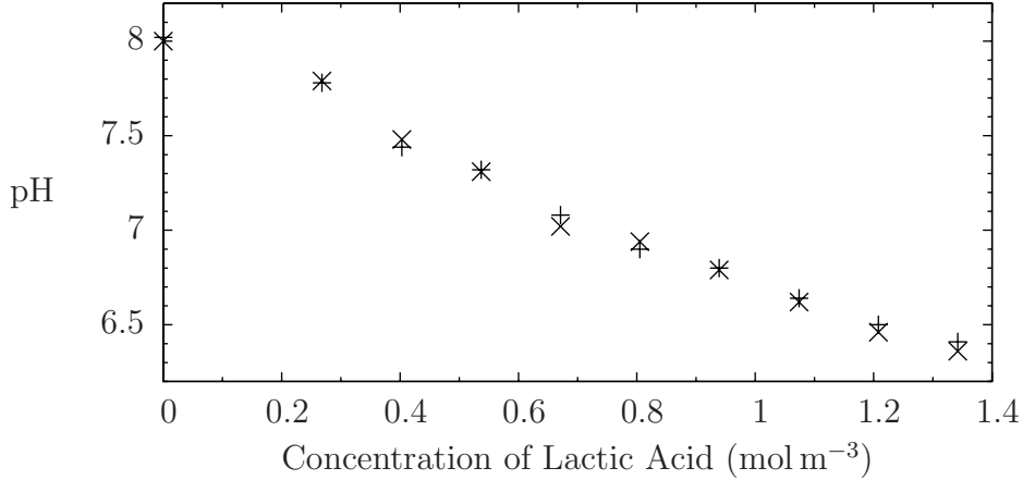
Fig. A.1. The results of two titrations lactic acid into a typical culture medium to assess the level of buffering present. The culture medium comprised D-MEM (Invitrogen, 2008) with 10% Fetal Calf Serum. Lactic acid was added drop-wise using a pipette, and data points comprising the volume added together with the pH of the solution were recorded. The agreement between the two titrations indicates good reproducibility.
