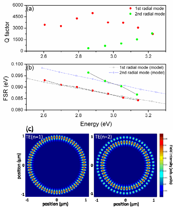
Fig. 3. (color online) The 1 st and the 2 nd radial order families of WGMs for a \sim 2 \mu\text{m} \mu -disk as these are indicated by a) their Q factor values and b) their free spectral range (FSR) (full circles). Theoretical values are shown in open circles. c) An example of simulated 1 st (left) and 2 nd (right) radial order modes for a 2.06 \mu\text{m} -diameter \mu -disk showing the TE field distribution within the disk plane.
