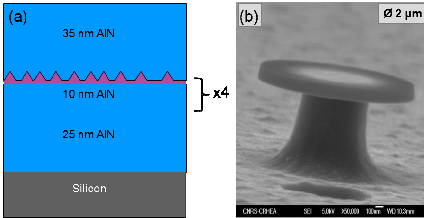
Fig. 1. (color online) a) Epitaxial structure: the optical active area above the Silicon substrate contains 4 periods of GaN/AIN QDs layers. b) SEM image of a 2 \mu\text{m} in diameter \mu -disk.
