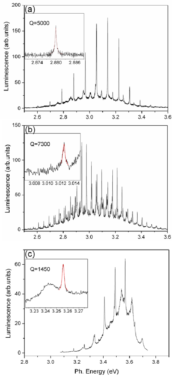
Fig. 2. (color online) Room temperature PL spectra of a),c) 2 \mu\text{m} and b) 5 \mu\text{m} in diameter \mu -disks with embedded a),b) GaN/AlN and c) GaN/AlGaIn dots presented within similar spectral range \sim 1.1 eV. Insets: High resolution spectra showing the WGM with the highest Q value.
