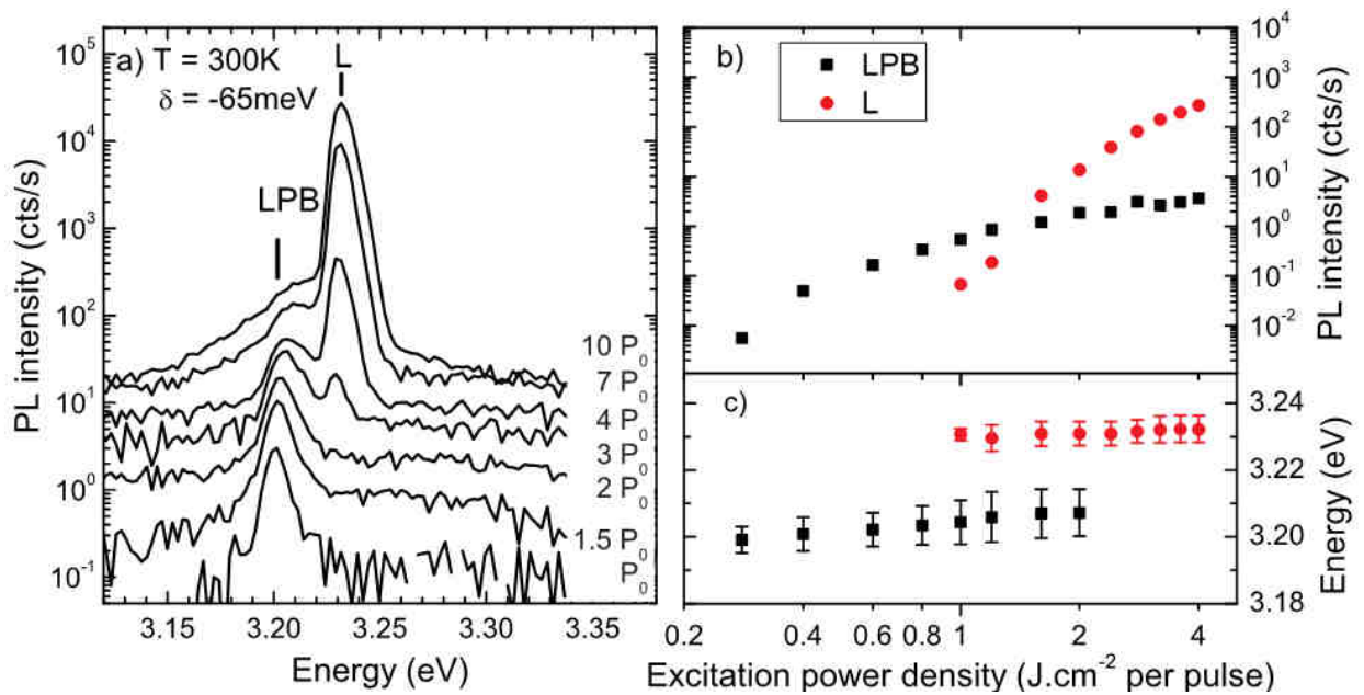
Figure 1 : (a) Photoluminescence at T=300 K and a detection angle of 0^\circ , as a function of the excitation power density ( P_0=0.4 \text{ J.cm}^{-2} per pulse); the lower polariton branch (LPB) and the lasing mode (L) are indicated; (b,c) Amplitude and energy of the two observed transitions.
