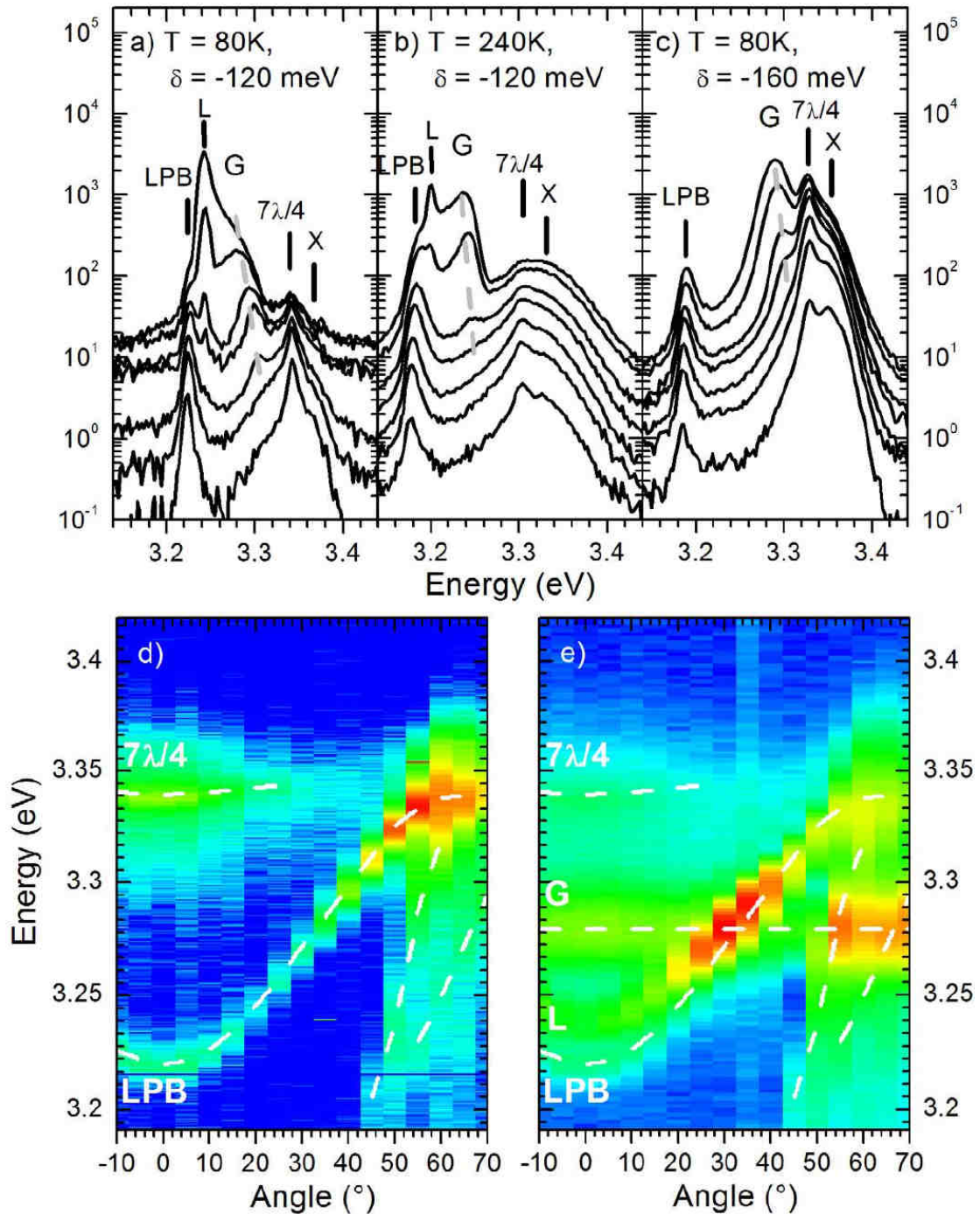
Figure 2 : a-c) Photoluminescence recorded at 0^\circ as a function of the excitation power density for various temperature and detuning conditions; the excitation power density increases from P_0 = 0.4\text{ J}\cdot\text{cm}^{-2} to 10 P_0 , similarly to Figure 1. The lower polariton branch (LPB), lasing mode (L), gain feature (G), 7\lambda/4 polariton mode ( 7\lambda/4 ) and exciton energy (X) are indicated. d,e) Angle-resolved photoluminescence spectra below (d, P = P_0 ) and above (e, P = 5 P_0 ) the lasing threshold, in the same conditions as in Figure 2.a; the PL intensity is represented in a logarithmic color scale. The dispersion of the LPB and 7\lambda/4 modes measured at low excitation power are indicated as dashed lines, as well as two Bragg modes visible at large angles and the L and G transitions appearing at large excitation power.
