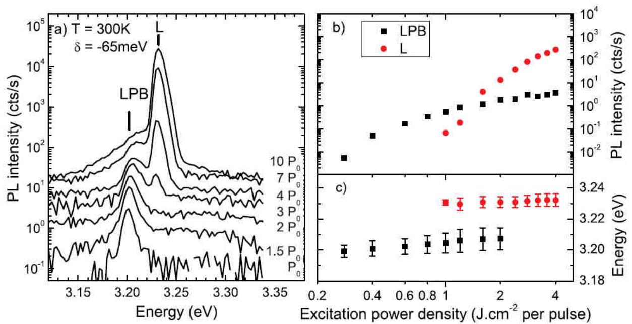
Figure 1 : a) Photoluminescence at T=300\text{ K} and a detection angle of 0^\circ , as a function of the excitation power density ( P_0=0.4\text{ J}\cdot\text{cm}^{-2} per pulse); the lower polariton branch (LPB) and the lasing mode (L) are indicated; b,c) Amplitude and energy of the two observed transitions.
