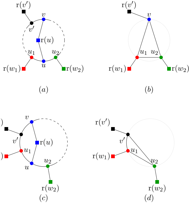
Figure 4: Illustration for Lemma 16.
