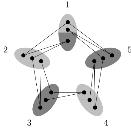
Figure 6: Illustration for Lemma 19, each ellipse represents a color.
