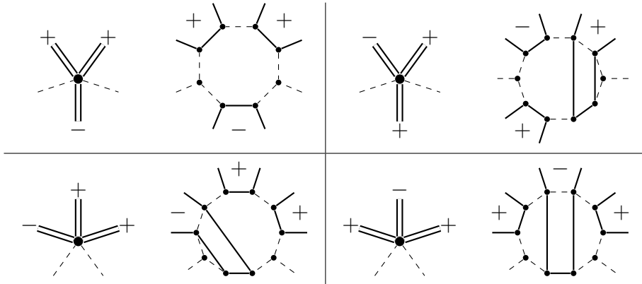
FIGURE 2. Variable gadgets.
