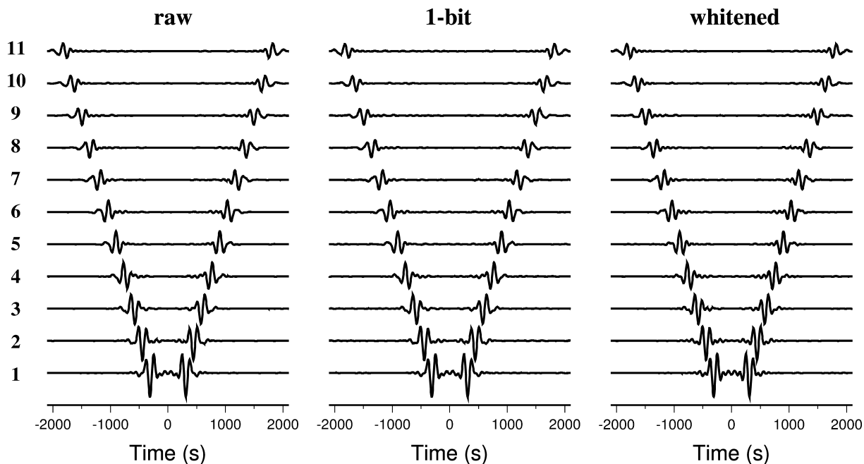
Figure 2. Cross-correlations between the vertical displacement recorded at 0 and the vertical displacement at n (numbers on the left) in the case of a uniform distribution of noise sources. Three data sets are presented corresponding to the three different noise processing investigated in this work: raw, one-bit normalization and whitening.
