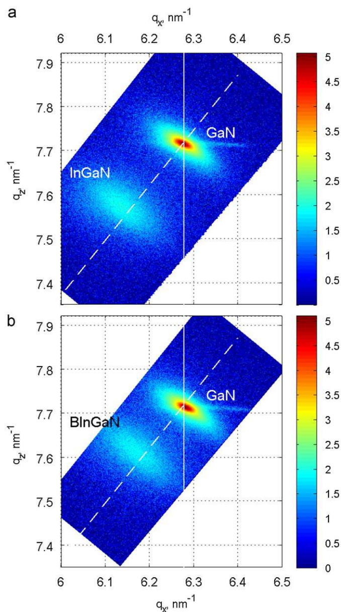
Fig. 2. Reciprocal space maps of the (11.4) diffraction of the InGaN and BInGaN samples grown on GaN template for (a) TEB=0 sccm and (b) TEB=3.27 sccm. Both samples demonstrate the complete relaxation of strain between the grown layer and the GaN substrate.
