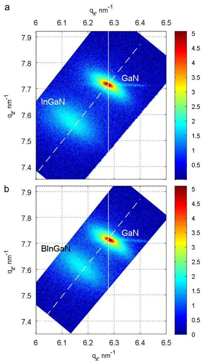
Fig. 2. Reciprocal space maps of the (1 1.4) diffraction of the InGaN and BInGaN samples grown on GaN template for (a) TEB=0 sccm and (b) TEB=3.27 sccm. Both samples demonstrate the complete relaxation of strain between the grown layer and the GaN substrate.
