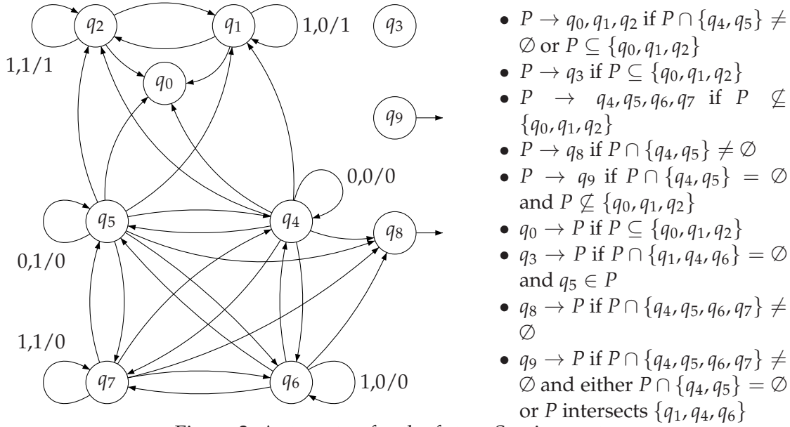
Figure 3: Automaton for the future Stavi operator
