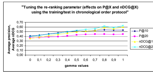
Fig. 3. Effect of the parameter gamma on Precision and nDCG in the combined ranks using the training/test in chronological order protocol.
