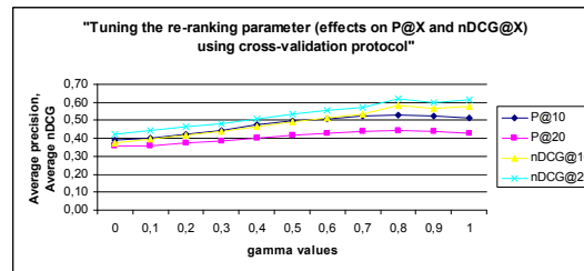
Fig. 4. Effect of the parameter gamma on Precision and nDCG in the combined ranks using the k-fold cross validation protocol.
