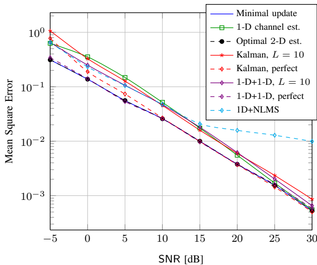
Fig. 2. MSE performance of the minimal update channel estimation against one-dimensional and two-dimensional (optimal) MMSE with K = 4 past pilot symbols, vehicular speed 120 km/h, LTE OFDM model.
