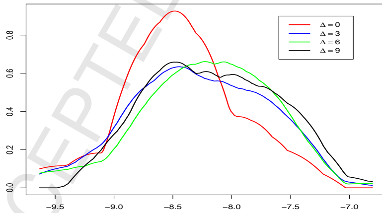
Figure 16: Predictive density of \log(IV_{T+1}) , conditional on \log(IV_{T-\Delta}) , for the Intel stock, based on \widehat{RV}_{t,e,M} . M = 2340 , T = 100 .
