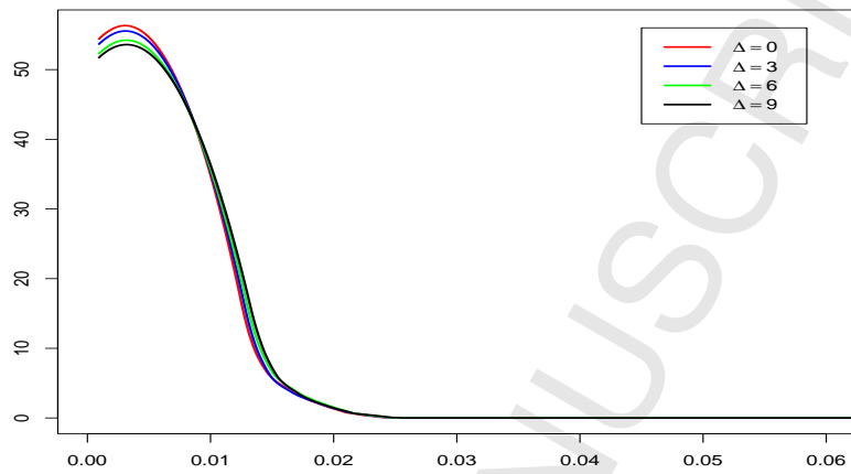
Figure 5: Predictive density of IV_{T+1} , conditional on IV_{T-\Delta} , for the Intel stock, based on realized volatility. M = 2340 , T = 100 .
