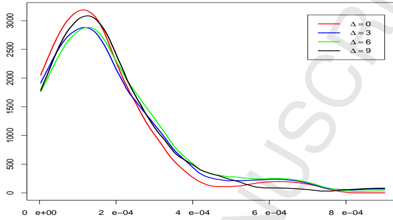
Figure 3: Predictive density of IV_{T+1} , conditional on IV_{T-\Delta} , for the Intel stock, based on \widehat{RV}_{t,l,M} . M = 78, T = 100 .
