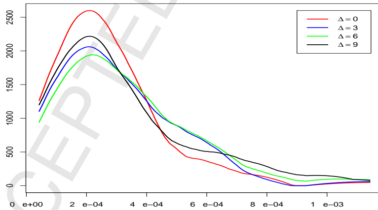
Figure 4: Predictive density of IV_{T+1} , conditional on IV_{T-\Delta} , for the Intel stock, based on \widetilde{RV}_{t,e,M} . M = 78, T = 100 .
