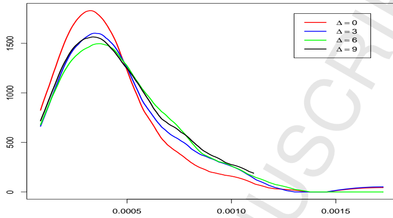
Figure 1: Predictive density of IV_{T+1} , conditional on IV_{T-\Delta} , for the Intel stock, based on realized volatility. M = 78 , T = 100 .
