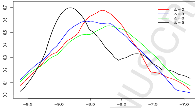
Figure 15: Predictive density of \log(IV_{T+1}) , conditional on \log(IV_{T-\Delta}) , for the Intel stock, based on \widehat{RV}_{t,l,M} . M = 2340 , T = 100 .
