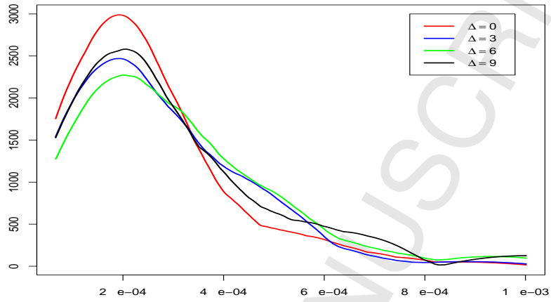
Figure 7: Predictive density of IV_{T+1} , conditional on IV_{T-\Delta} , for the Intel stock, based on \widehat{RV}_{t,l,M} . M = 2340 , T = 100 .
