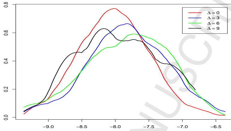
Figure 9: Predictive density of \log(IV_{T+1}) , conditional on \log(IV_{T-\Delta}) , for the Intel stock, based on realized volatility. M = 78 , T = 100 .
