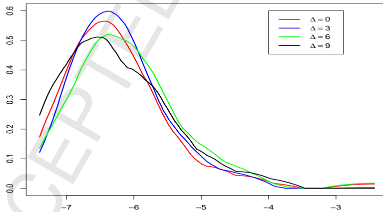
Figure 14: Predictive density of \log(IV_{T+1}) , conditional on \log(IV_{T-\Delta}) , for the Intel stock, based on bipower variation. M = 2340 , T = 100 .
