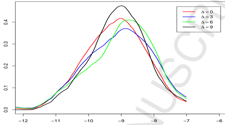
Figure 11: Predictive density of \log(IV_{T+1}) , conditional on \log(IV_{T-\Delta}) , for the Intel stock, based on \widehat{RV}_{t,l,M} . M = 78 , T = 100 .
