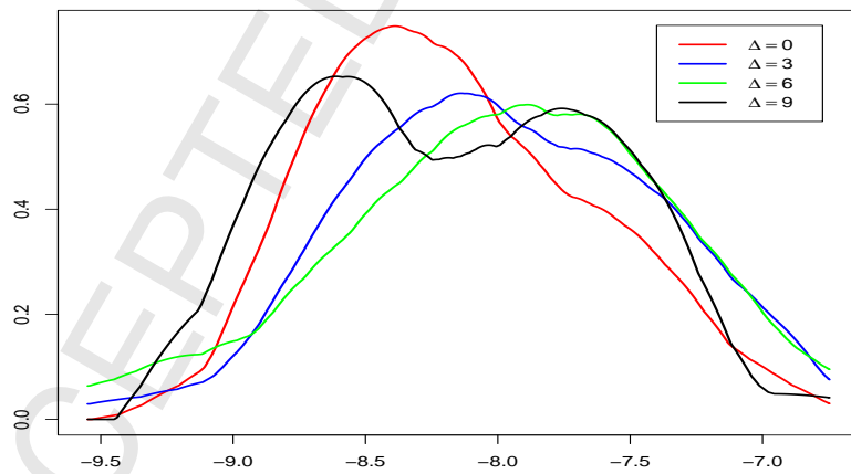
Figure 10: Predictive density of \log(IV_{T+1}) , conditional on \log(IV_{T-\Delta}) , for the Intel stock, based on bipower variation. M = 78 , T = 100 .
