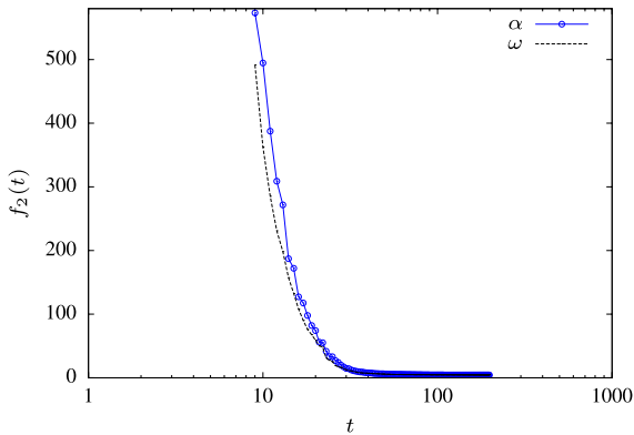
Fig. 7 Evolution of the Colville function, with variable \alpha and \omega
