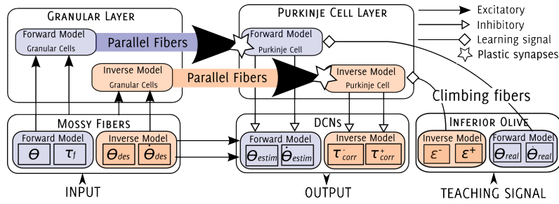
Fig. 2. The cerebellar microcomplex model.
