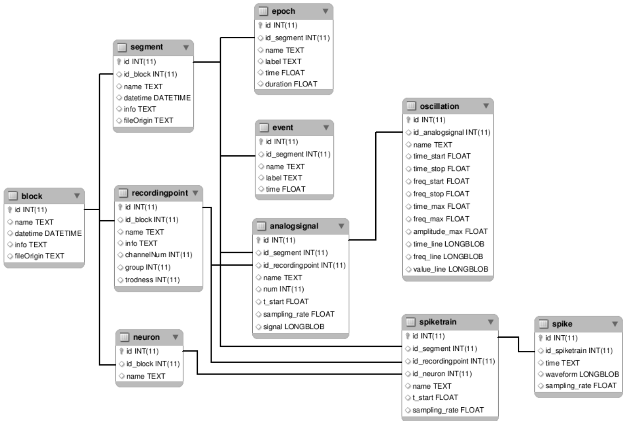
Figure 1: Database scheme. It presents the different tables and fields present in the database. The lines represent the relationship between tables by linking the related indices. For example, each member of the table recordingpoint is part of a block, and contains analogsignals and spiketrains.
