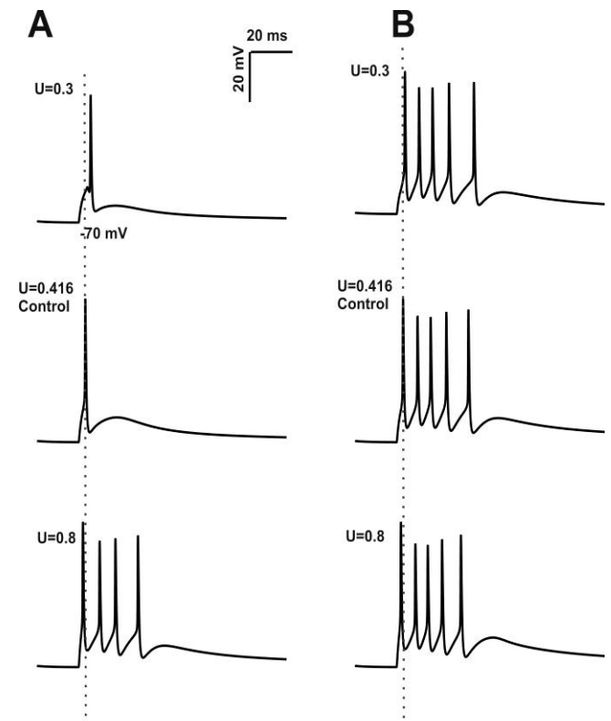
Figure 1. Changes in Mossy fibre release probability. A. EPSP obtained by in vitro like input through 4 MF synapses, 2 inhibitory synapses of granule cell with varying release probability. First spike latency was reduced (see the grey dotted line) and number of spikes was increased by the increase in release probability. B. 4 MF synapses, 2 inhibitory synapses activation of granule cell in vivo with changes in release probability. At U=0.1 , change in initial spike delay and decrease in number of spikes was clearly observed. During control condition ( U=0.416 ), increase in number of spikes and shortening of first spike latency was seen (the grey dotted line passing through the centre of first spike). When the release probability of excitatory synapses was increased to 0.8, number of spikes remains constant, small change in initial spike latency was seen.
