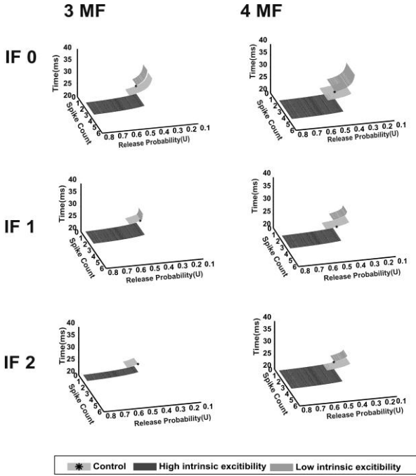
Figure 5. Quantifying information transfer in spiking neurons for single spike ( in vitro ) input. Light grey region shows number of spikes, first spike delay for release probability changes ( U=0.35-0.45 ). Black dot (over light grey) shows the control ( U=0.416 ) value. Black area shows model variation with high intrinsic excitability. The grey area shows model with low intrinsic excitability. X axis indicated various release probabilities; Y-axis shows number of spikes, Z-axis shows first spike latency (ms). MF: Mossy Fiber Synapses, IF: Inhibitory Fibre.
