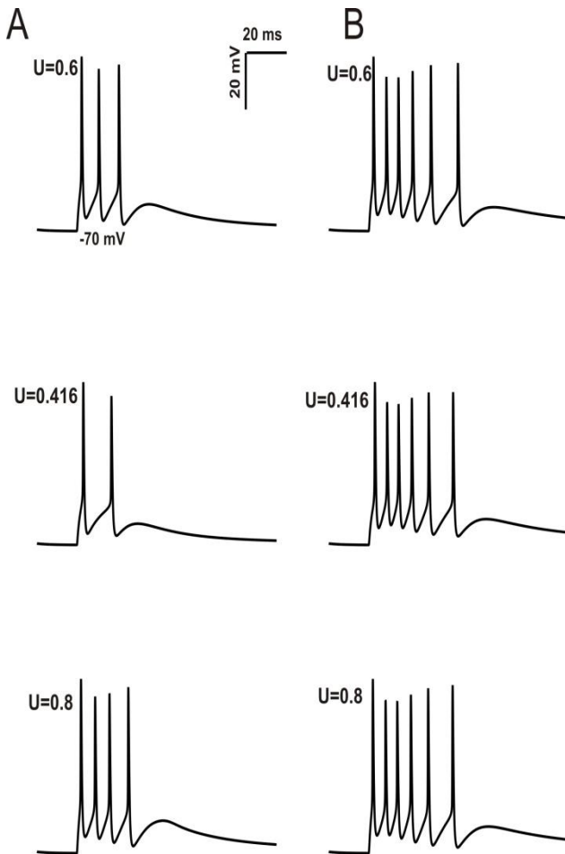
Figure 2. Simulating LTP A. 1 inhibitory synapse 4 excitatory synapses activating granule cell with high intrinsic excitability. Varying release probability of mossy fibre for single spike input shows difference in number of spikes A. Single spike input via MF B. Burst like input via MF. Note the number of spikes remains constant.
