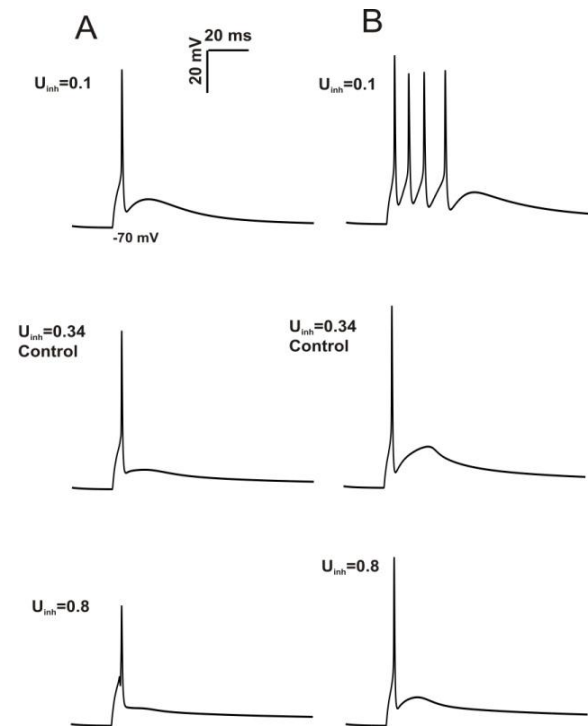
Figure 4. Spiking characteristics of granule cell with single and burst as input. For in vitro like behaviour first spike delay was reduced with lesser inhibition. The first spike delay remains constant irrespective of the release probability change in inhibitory synapses for in vivo like behaviour.
