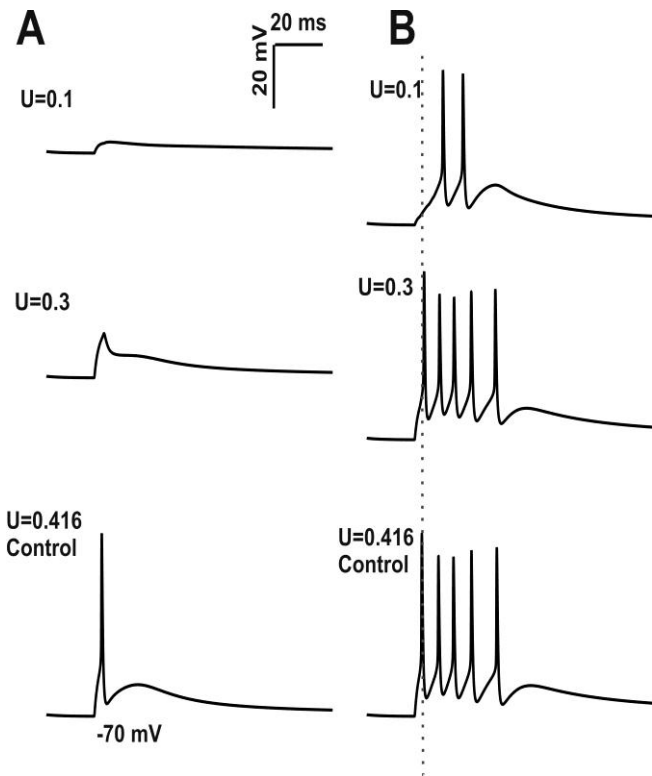
Figure 3. Simulations of changes in mossy fibre release probability and intrinsic excitability. A. In vitro behaviour of granule cell model with low release probabilities of MF synapses B. in vivo behaviour of granule cell model during low release probability of mossy fibre. First spike latency was increased when there was a reduction in MF synapse release probability coupled with low intrinsic excitability of granule cell (see grey dotted line passing through control). It can be noted that the decrease in release probability of MF synapses was associated with decrease in number of spikes.
