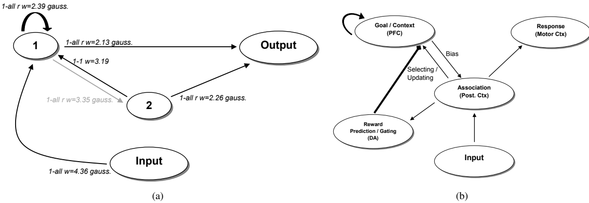
Figure 2. (a) Example of a module obtained with map-based neuroevolution. In this case, each map is composed of 4 neurons. 1-1 represents one to one connections between maps, 1-all, one to all connections, gauss., weights following a gaussian distribution; (b) Minimalist canonical model of cognitive control proposed by Braver [9]
