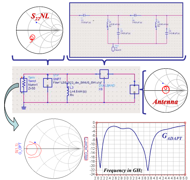
Fig. 2 : Optimization of loading network, with extraction of transistor S_{22NL} , polarization inductance and antenna load. Resulting G_{ADAPT} .
