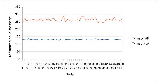
Fig. 8. Number of HELLO messages per node
