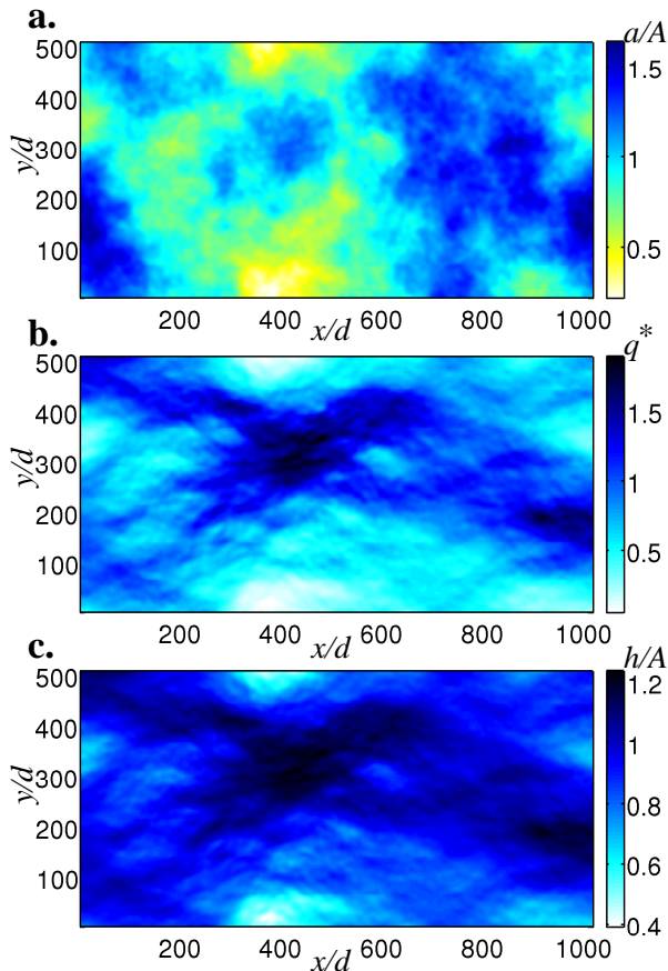
Figure 4: (Color online) a.: Self affine aperture with \sigma/A = 0.25 . b.: Dimensionless hydraulic flow norm computed with the aperture of Fig. 4a., having for dimensionless hydraulic aperture H^* = 0.94 . c.: Microscopic hydraulic apertures, computed from the third root of the hydraulic flow shown in Fig. 4b.
