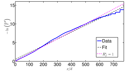
Figure 12: (Color online) Continuous curve: -\ln(\overline{\overline{T}}^*) , opposite of the logarithm of the temperature field computed from the temperature field \overline{T} shown in Fig. 9. Dash-dotted curve: Linear fit of curve A (from x/d = 0 to x/d = 772 ), which provides the thermal length: -\ln(\overline{\overline{T}}^*) = x/1.09 + 0.6 , i.e. R^* = 1.09 . Dashed curve: -\ln(\overline{\overline{T}}_{//}^*) opposite of the logarithm of the temperature law for the same fracture modeled without self-affinity perturbation ( i.e. parallel plates), which has for thermal length R_{//}^* = 1 .
