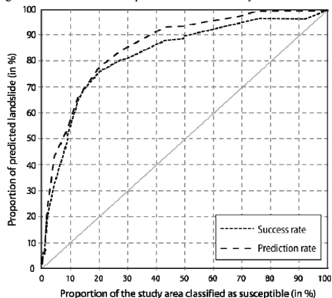
simulation 3 (final susceptibility map).
