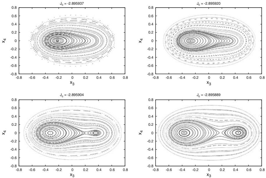
Fig. 21 For \delta = 0.01 ; Poincaré sections for x_2 = 0 for different \hat{J}_C . From left to right, top to bottom \hat{J}_C = -2.895937, -2.895920, -2.895904, -2.895889
