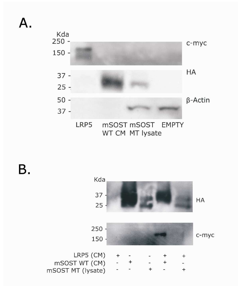
36 37 38 39 40 41 42 43 44 45 46 47 48 49 50 Figure 4. Impaired binding of MT sclerostin to LRP5. A. Total cell lysates and CM from HEK293T cells transfected with WT or MT SOST were analyzed for the expression of HA-tagged sclerostin by immunoblotting using HA antibodies. Expression of LRP5-myc protein in CM was evaluated by immunoblotting with c-myc antibodies. A negative control (empty pcDNA3.1) was included in both immunoblotting experiments. Equal protein loading was confirmed by immunoblotting of total cell lysates for \beta -actin. B. Mixtures of CM containing truncated WT-LRP5-myc and either CM containing WT-sclerostin-HA (lane 4) or cell lysates containing MT-sclerostin-HA (lane 5) were immunoprecipitated using EZ-view™ Red Anti-HA affinity gels. Cells that were transfected only with LRP5-myc (lane 1) or WT and MT SOST -HA expression vectors (lane 2-3) were used as controls. Immunodetection of HA-immunoprecipitated protein was performed with both anti-HA and anti-myc. From lane 4 and 5 it is clear that WT but not MT sclerostin-HA was able to precipitate LRP5-myc.
