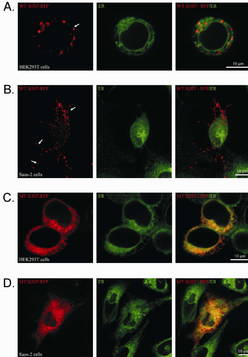
Figure 2. Retention of MT sclerostin in the ER. A-B. HEK293T ( A ) and Saos-2 cells ( B ) were transiently transfected with WT SOST -RFP plasmid to study the subcellular localization of WT mouse sclerostin ( red channel). ER staining was performed using a green fluorescent ER tracker ( green channel). Living cells were viewed using an UltraVIEW dual spinning disk confocal system. Arrows indicate the presence of WT sclerostin in variably sized granular cytoplasmic structures, preferentially in areas close to the cell membrane. The ER networks typically showed the highest density around the nucleus. Merging of the red and green channels clearly revealed that both labels are not co-localized. The latter was most obvious in the many cytoplasmic processes of Saos-2 cells. C-D. Similar to Figure 4 A-B, but now HEK293T ( C ) and Saos-2 cells ( D ) were transfected with MT SOST -RFP. The orange/yellow color in the merged channel images revealed a major co-localization of MT SOST protein with the ER tracker in both cell types. Scale bars are indicated.
