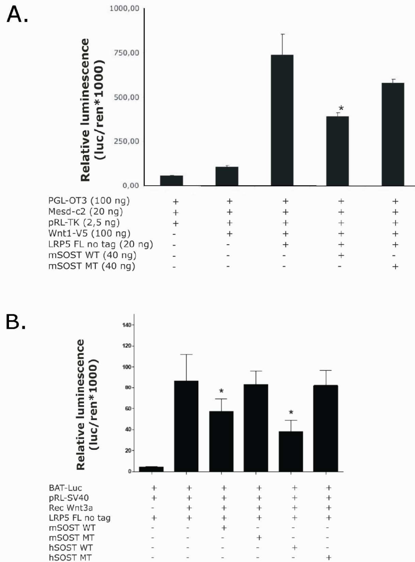
Figure 3. Decreased level of Wnt signal transduction both in the presence of human and mouse MT sclerostin. A. Saos-2 cells were transiently transfected with pGL3-OT, pRL-TK, Mesdc2 , untagged full length WT- LRP5 in the presence or absence of Wnt1-V5 . The antagonistic activity on Wnt signaling was evaluated by co-transfecting either WT or MT mSOST . Data were generated in three independent experiments, each performed in triplicate. Bars represent mean values \pm SD. * p < 0.05 cells transfected with WT mSOST compared to cells transfected without WT mSOST . B. Saos-2 cells were transfected with untagged full length WT- LRP5 and BAT-luc with or without mouse and human WT or MT SOST expression vectors and stimulated with rec Wnt3a 24h after transfection (n=8). Bars represent mean values \pm SD. * p < 0.05 cells transfected with mouse or human WT SOST compared to cells transfected without mouse or human WT SOST . All data were corrected for differences in transfection efficiency by co-transfection with constitutively active Renilla -luciferase expression plasmids.
