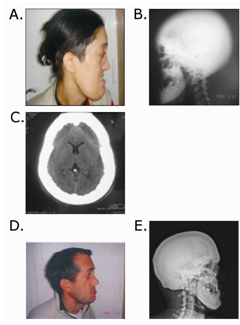
Figure 1. A. Lateral view of the female patient's face showing a marked mandibular prognathism. B. Plain radiograph of the skull (lateral view) showing uniform sclerosis of the calvaria, skull base and facial bones (particularly the mandible). C. Axial CT-scan of the brain showing marked thickening of the cranial vault. D. Lateral view of the face of the female's brother, who also shows a marked mandibular prognathism. E. Plain radiograph of the skull (lateral view) of the brother, showing uniform sclerosis of the skull and the mandible.
