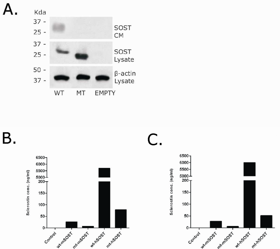
Supp. Figure S1. Decreased intra- and extracellular levels of MT sclerostin. A. Total cell lysates and CM from HEK293T cells transfected with WT or MT SOST or empty vector were analyzed for the expression of HA-tagged sclerostin by immunoblotting using an HA antibody. Equal protein loading was confirmed by immunoblotting of total cell lysates for \beta -actin. One representative experiment of three independent immunoblotting experiments is depicted. B. Quantitative expression analysis of sclerostin in cell lysates of HEK293T cells transfected with WT and MT constructs of both mouse and human SOST or an empty control vector using the MULTI-ARRAY ® Human sclerostin assay (MSD). Sclerostin levels were corrected for SOST mRNA expression levels for each of the plasmids determined by RT-PCR analysis. C. Same in CM of transfected HEK293T cells.
