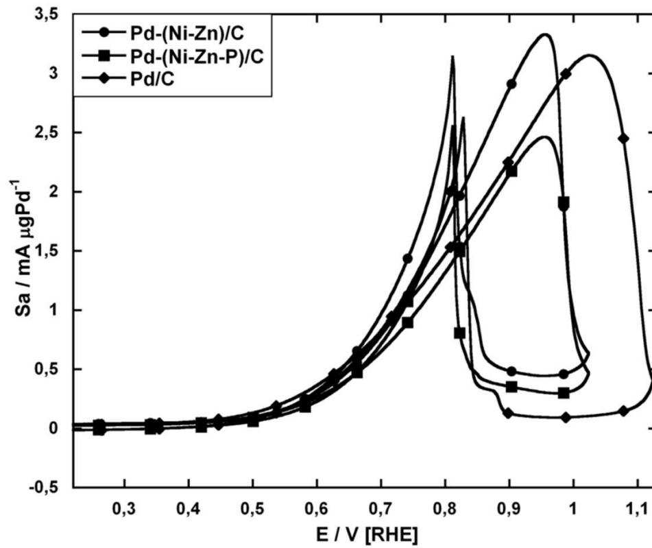
Figure 4. Cyclic voltammograms (at the tenth cycle) of EG oxidation on Pd-(Ni-Zn)/C, Pd-(Ni-Zn-P)/C and Pd/C electrodes in 2 M KOH and 5 wt% EG. Scan rate: 50 \text{mV s}^{-1} . 74x65mm (400 x 400 DPI)
