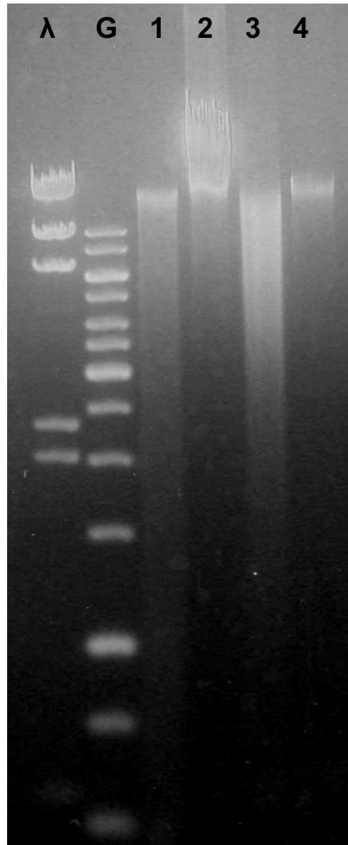
Figure 1: Comparison of P. pastoris gDNA quality of diverse isolation methods. G: GeneRuler 1kb (Fermentas), λ: λ-HindIII Standard (Fermentas), 1: 5 μL of gDNA isolated using Y-PER (Novagen) and chloroform/phenol extraction followed by ethanol precipitation, 2: 5 μL of gDNA isolated according to Easy DNATM-Kit (Invitrogen), 3: 5 μL of gDNA isolated using a E.Z.N.A.® Yeast DNA Kit, 4: 5 μL of gDNA isolated using glass beads and phenol/chloroform extraction as described by Hoffmann and Winston [23]. 86x208mm (300 x 300 DPI)
