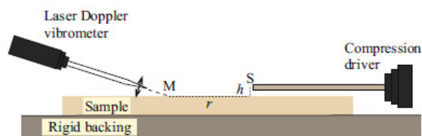
Figure 8. Experimental setup for measuring the shear modulus from the quarter wavelength resonance in a layer. (from ref [16])
