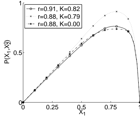
Fig. 5. Pressure distribution x_1 \mapsto p(x_1, x_2^0) , following the streamline x_2^0 := D/2 , in the (linear) converging profile. Influence of the elongation number (other parameters are: a = 0.80 , \widetilde{De} = 0.72 )
