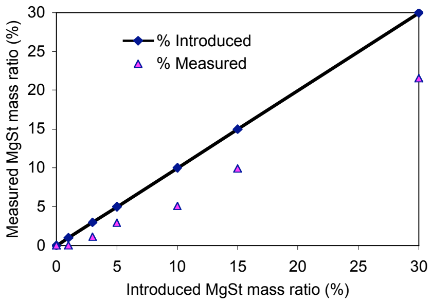
Fig. 6: Real mass fraction of MgSt 2 after the coating process calculates from the mass loss.
