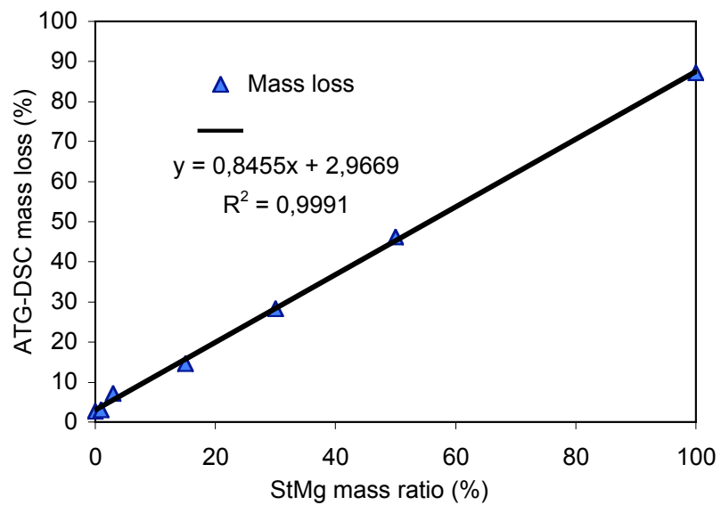
Fig. 5: Experimental relation between the TG-DSC mass loss (from 250°C to 600°C) and the mass ratio of MgSt_2 .
