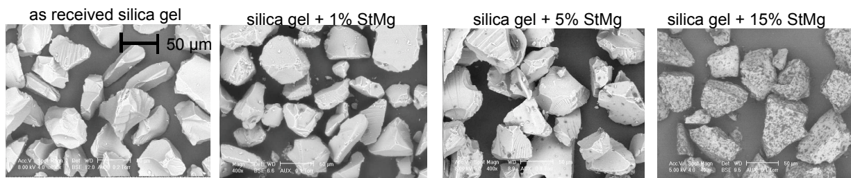
Fig. 2: ESEM images of silica gel and MgSt 2 -silica gel coated particles.
