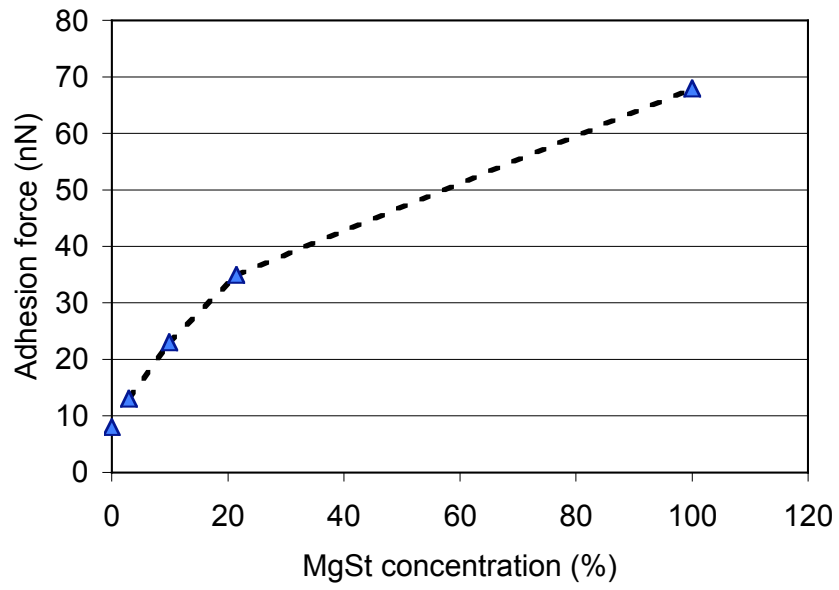
Fig. 10: Mean adhesion force (nN) as a function of the sample MgSt 2 concentration.
