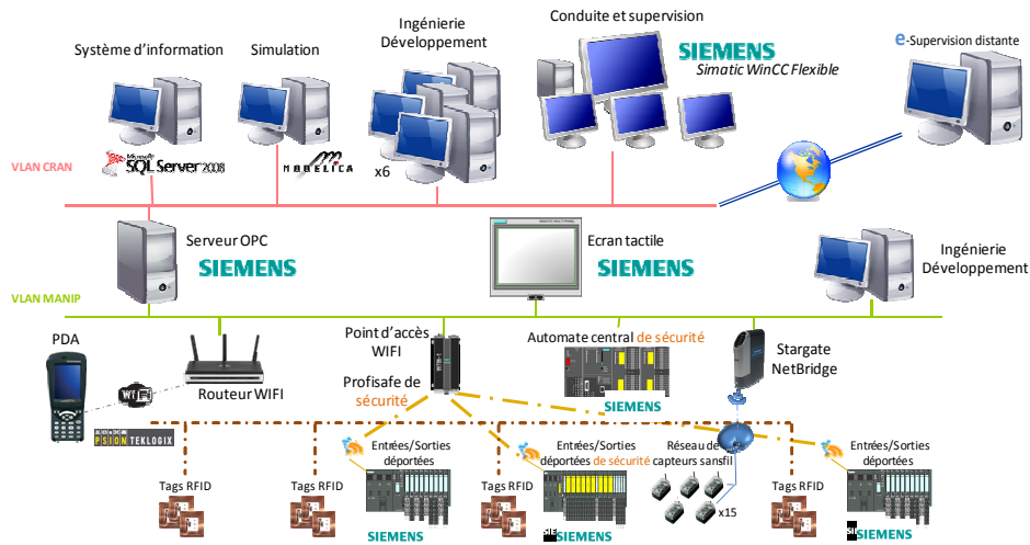
Figure 5 : Architecture de communication
