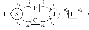
Figure 1. A Simple Stream Graph: the split node S consumes alternatively p_1 and p_2 elements from I . These are passed to filters F and G (that may be scheduled concurrently) and their outputs are combined by the join node J and passed to H .
