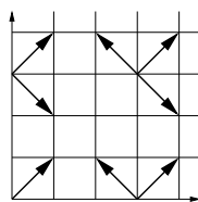
Figure 2: Walk considered in [12]
