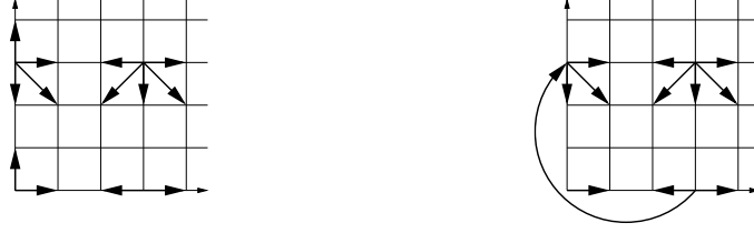
Figure 5: Two walks with different boundary behavior
