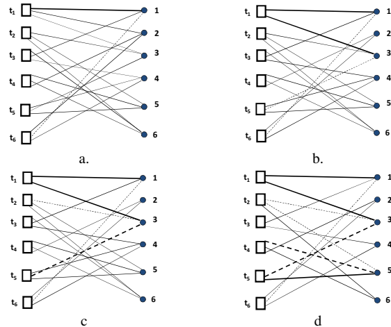
Figure 6: Path construction through Partitioning Algorithm
