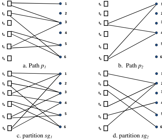
Figure 7: Path construction through Partitioning Algorithm
