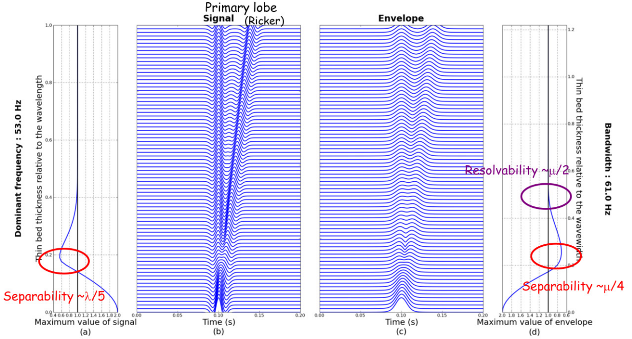
Figure 2: Thin bed response with identical-polarity reflections. (b) the seismic traces associated to the real signal. (c) the seismic traces associated to the envelopes of the signal. (a) the variation of the maximum value of the real signal as a function of a dimensionless parameter defined by the ratio of the bed thickness to the wavelength. (d) the variation of the maximum value of the envelope as a function of a dimensionless parameter defined by the ratio of the bed thickness to the “wavelength”. The signal is a 50Hz Ricker wavelet.
