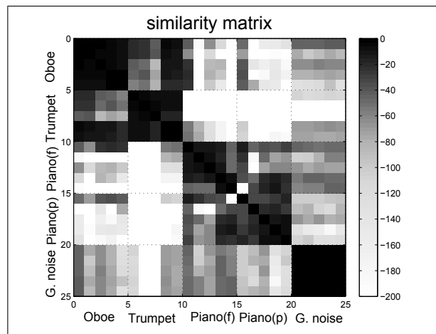
Figure 4: Similarity matrix computed with the measure \mu_s .
