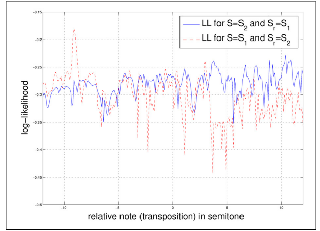
Figure 3: L_{A^2}(\lambda) as a function of 12 \log_2(\lambda) (pitch transposition in semitones) - dashed red plot: for S = S_1 (spectrum of 100ms frame of a piano A\#2 ) and S_r = S_2 (spectrum of 100ms frame of a piano C\#2 ). - plain blue plot: for S = S_2 and S_r = S_1 .
