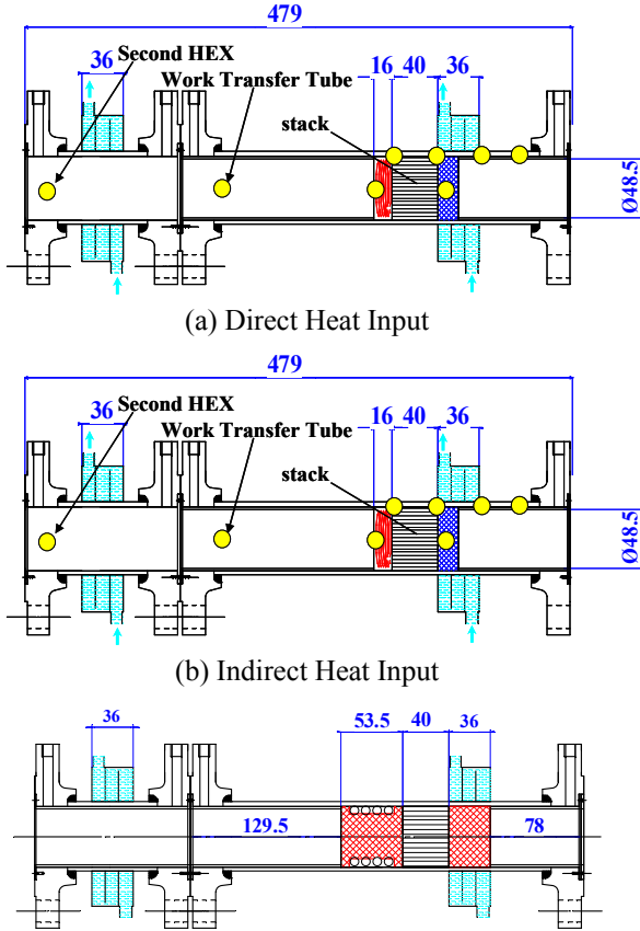
(a) Direct Heat Input (b) Indirect Heat Input (c) Semi-direct Heat Input Fig.2 Detail View of Stack Unit
