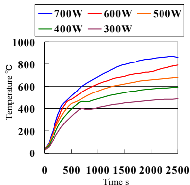
Fig. 9 Temperature History at Hot Side
