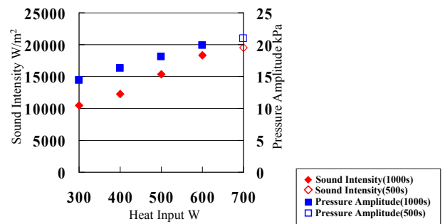
Fig.10 Sound Intensity, Pressure Amplitude vs. Heat Input
