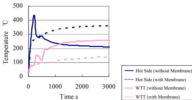
Fig.5 Temperature History(With & Without Membrane)
