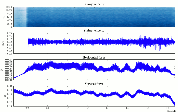
Figure 6: Rasping, appearing as almost pure noise, in the DWG model when touching very lightly.
