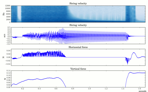
Figure 5: Spectrogram, velocity, and force plots of a bow stroke, actively damped at the end, using the DWG model running at 24 kHz with the body filter removed, string tuned to 80 Hz.
