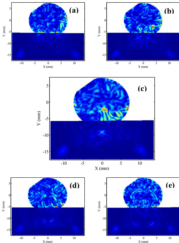
Figure 11: Calculated snapshots of the particle velocity at (a) t = 97.3 \mu\text{s} , (b) t = 98.3 \mu\text{s} , (c) t = 99.2 \mu\text{s} , (d) t = 100.4 \mu\text{s} , and (e) t = 101.4 \mu\text{s} for a copper chaotic cavity glued on a non reverberating composite sample.
