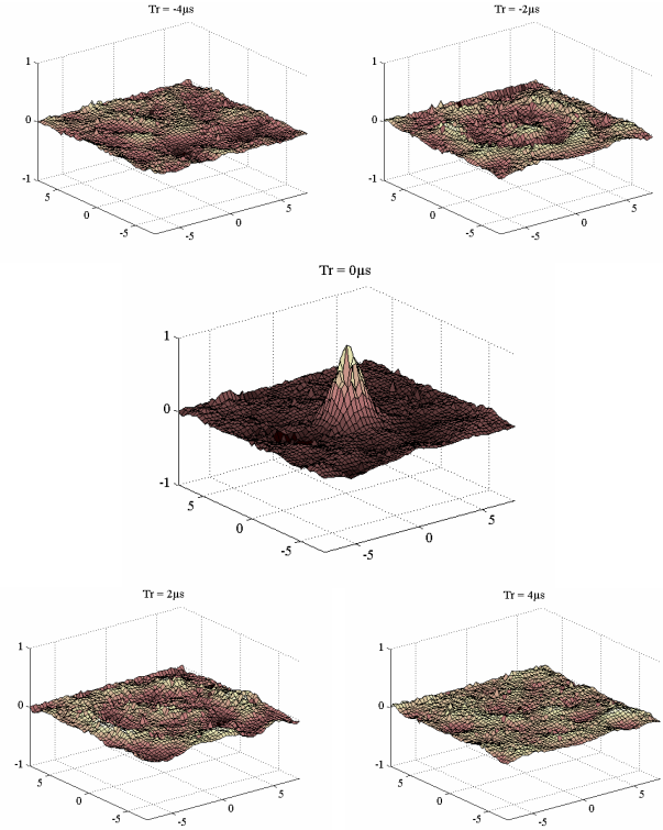
Figure 7: Snapshots of the surface particle velocity around the focal point at different moments of time showing the IF focalization obtained with a “chaotic cavity transducer”.
