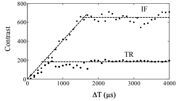
Figure 4: Contrast of the retro-focalised signal for Time Reversal (TR) and Inverse Filter (IF) processes.
