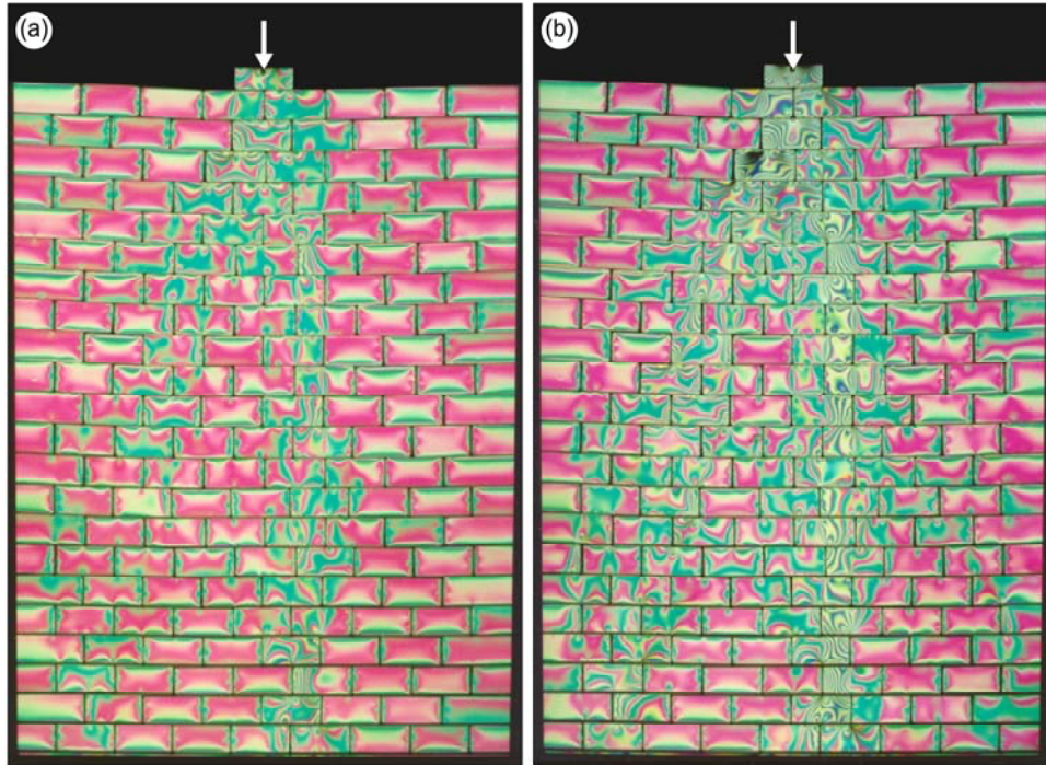
Fig. 7 – Photoelastic fringes of a model of dry masonry detected with a linear transmission polariscope at white light with analyzer inclined at 45^\circ . Material used is Lexan ® (the white arrow denote the applied vertical load). (a) low vertical load (400 N); (b) high vertical load (800 N).
