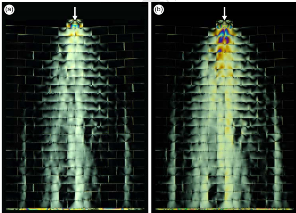
Fig. 8 – Photoelastic fringes of a model of dry masonry detected with a linear transmission polariscope at white light with analyzer inclined at 45^\circ . Material used is PMMA (the white arrow denote the applied vertical load). (a) low vertical load (1000 N); (b) high vertical load (2500 N).
