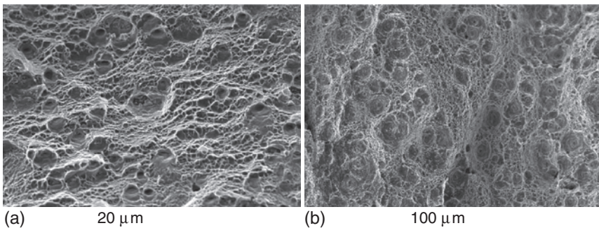
Figure 2. Examples of ductile failure involving two populations of cavities. (a) Al 2024 (Bron, 2004) secondary voids are nucleated on dispersoid particles having a typical size between 0.05 and 0.5 μm. These particles contain Zr, Mn, or Cr. (b) X100 steel (Luu, 2006): secondary voids are nucleated on Fe 3 C carbides.
