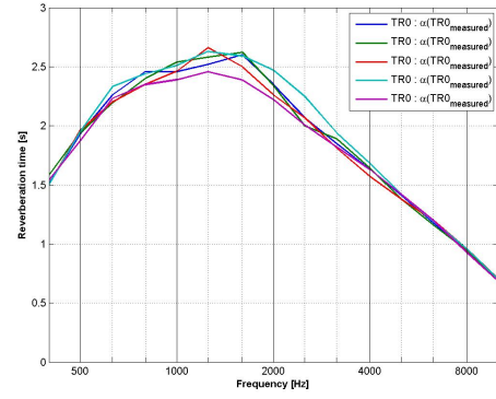
FIGURE 11 – Simulated Reverberation Times : 5 microphone positions
