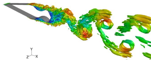
Figure 5: Flow topology of the two grooves configuration katana blade described by the Q-factor.
